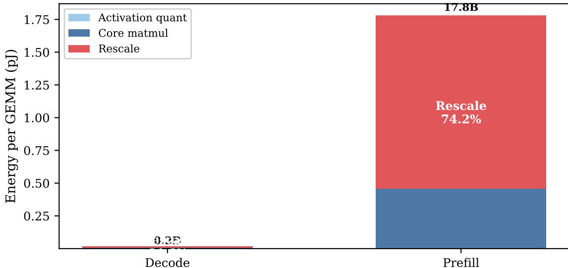
1e10 W4A4 Inference Energy Breakdown by Workload Regime
